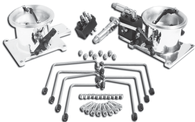
Single/Dual Butterfly Injector
