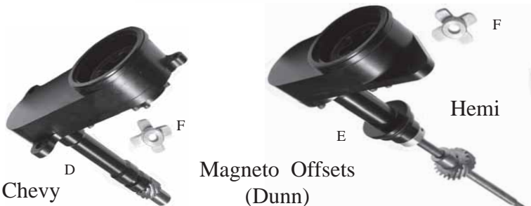
Front Pump/ Magneto Drive (RCD)
